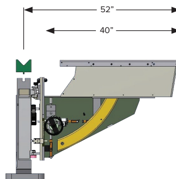
Sheet Extender
